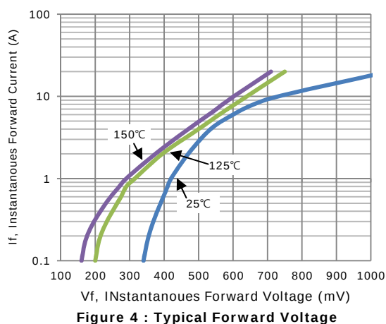
Figure 4 : Typical Forward Voltage
