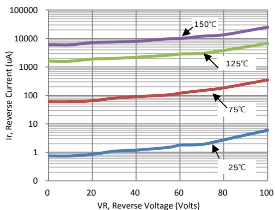
Figure 3 : Typical Reverse Current
